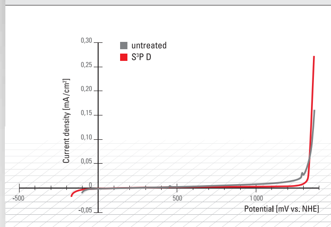
Current density-potential curve of the standard duplex steel 1.4462 in 3% NaCl solution. S 3 P maintains the excellent corrosion resistance of 1.4462 duplex stainless steel.
