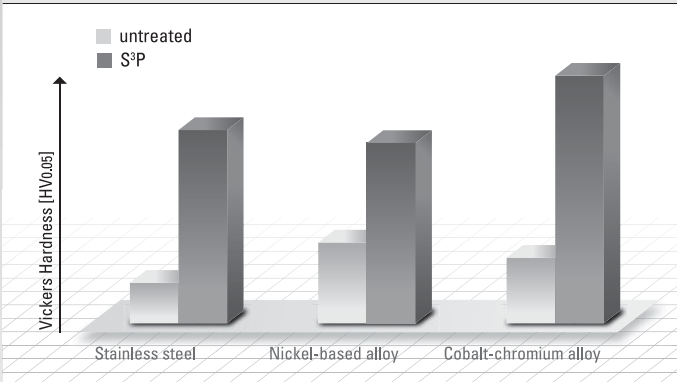
Comparing the surface hardness, S 3 P-treated materials show higher levels of hardness, resulting in improved wear resistance.
