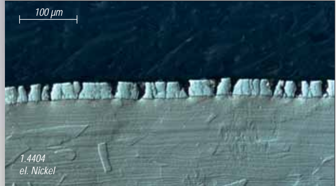
Fig. 1 Cracks in electroless nickel plating on AISI316L after slight bending.
