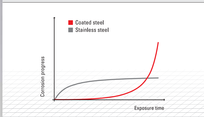
Fig. 1 Different mechanisms of coated steel and stainless steel in salt spray test (ISSF, 2008).
