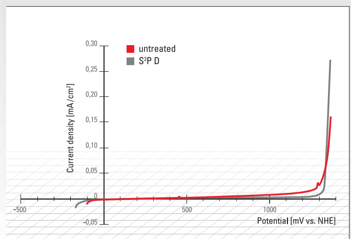
Summation-current density-potential curve of the standard duplex steel 1.4462 in 3% NaCl solution. S 3 P maintains the excellent corrosion resistance.
